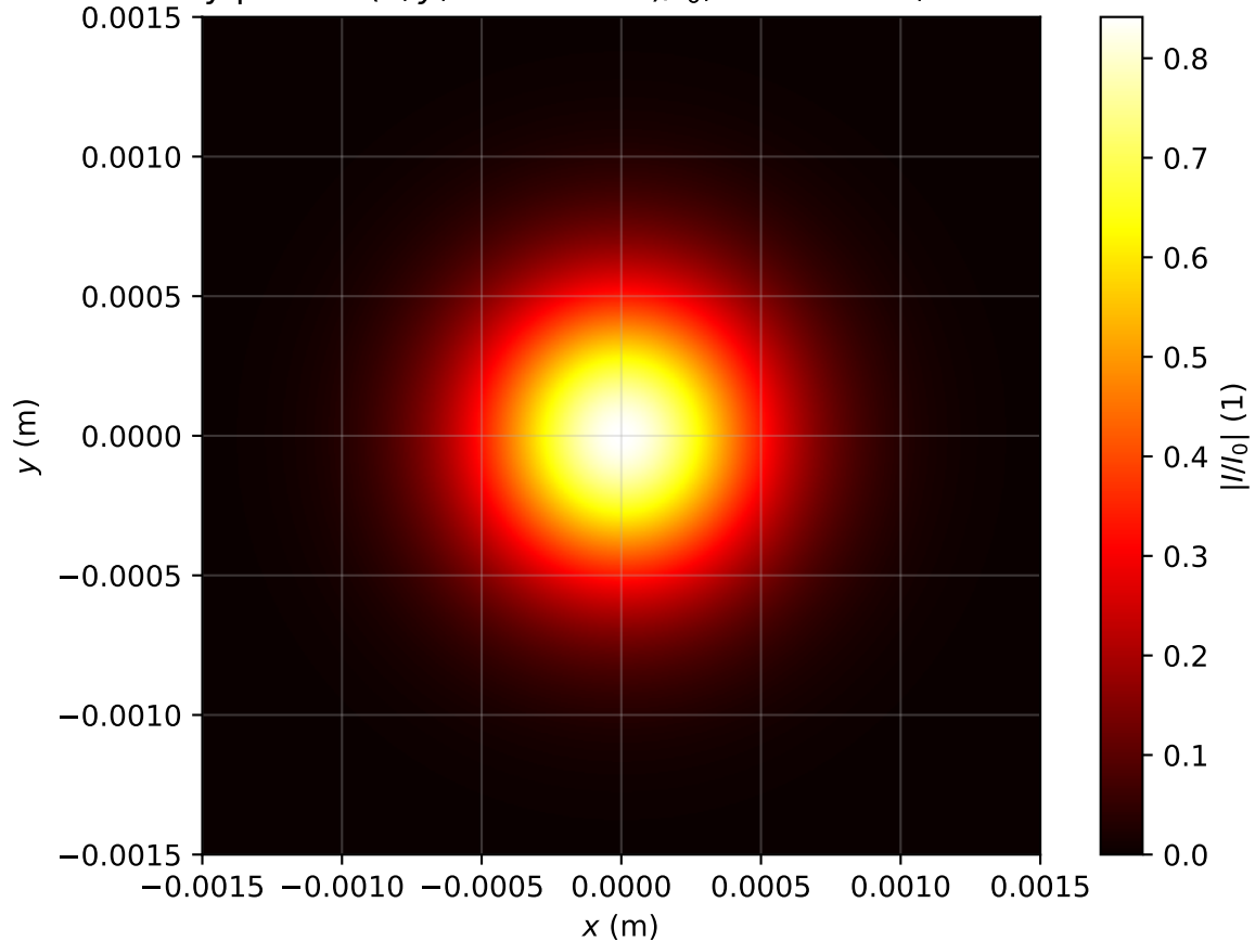
Intensity profile I(x, y, z = 1.353m)/I_0 , Pin=0.3Pcr, artificial time
